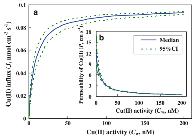
Fig. 2 Cu(II) influx and permeability across gill membrane of C. fluminea as the function of waterborne Cu(II) ranging from 0–200 nM. a Cu(II) influx based on M–M kinetics (Eq. (9)). b Cu(II) permeability across gill membrane
